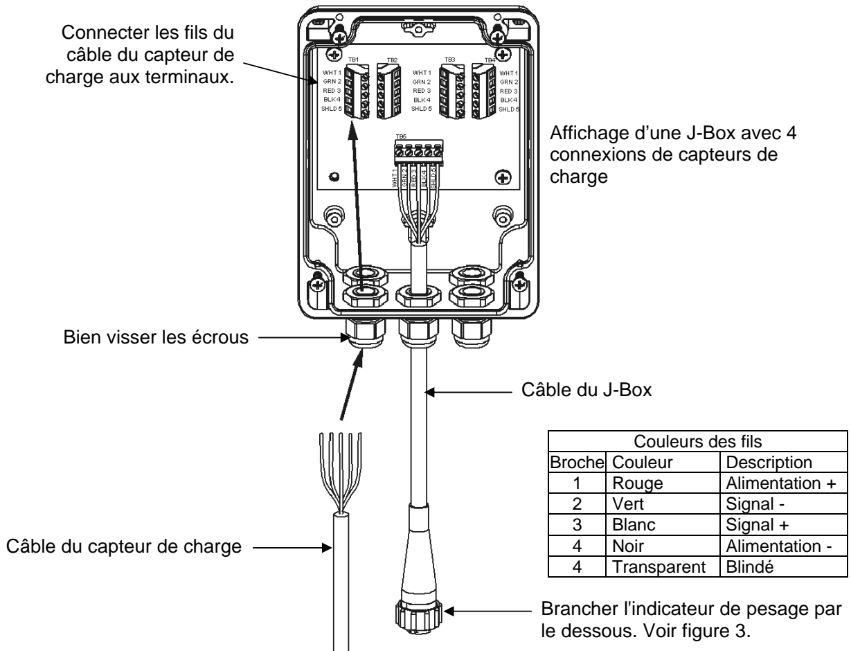
Figure 4 : Branchements J-Box
